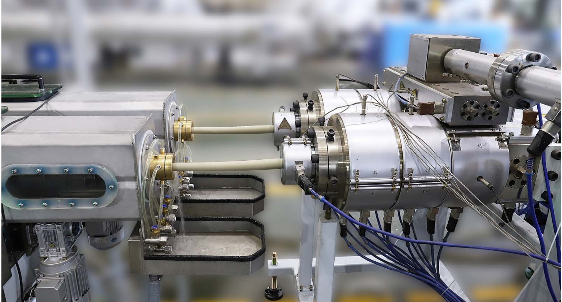
Three Layer ABA structure, Dual Pipe Head
